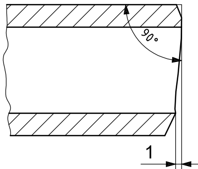
Figure 3 — Out-of-squareness
