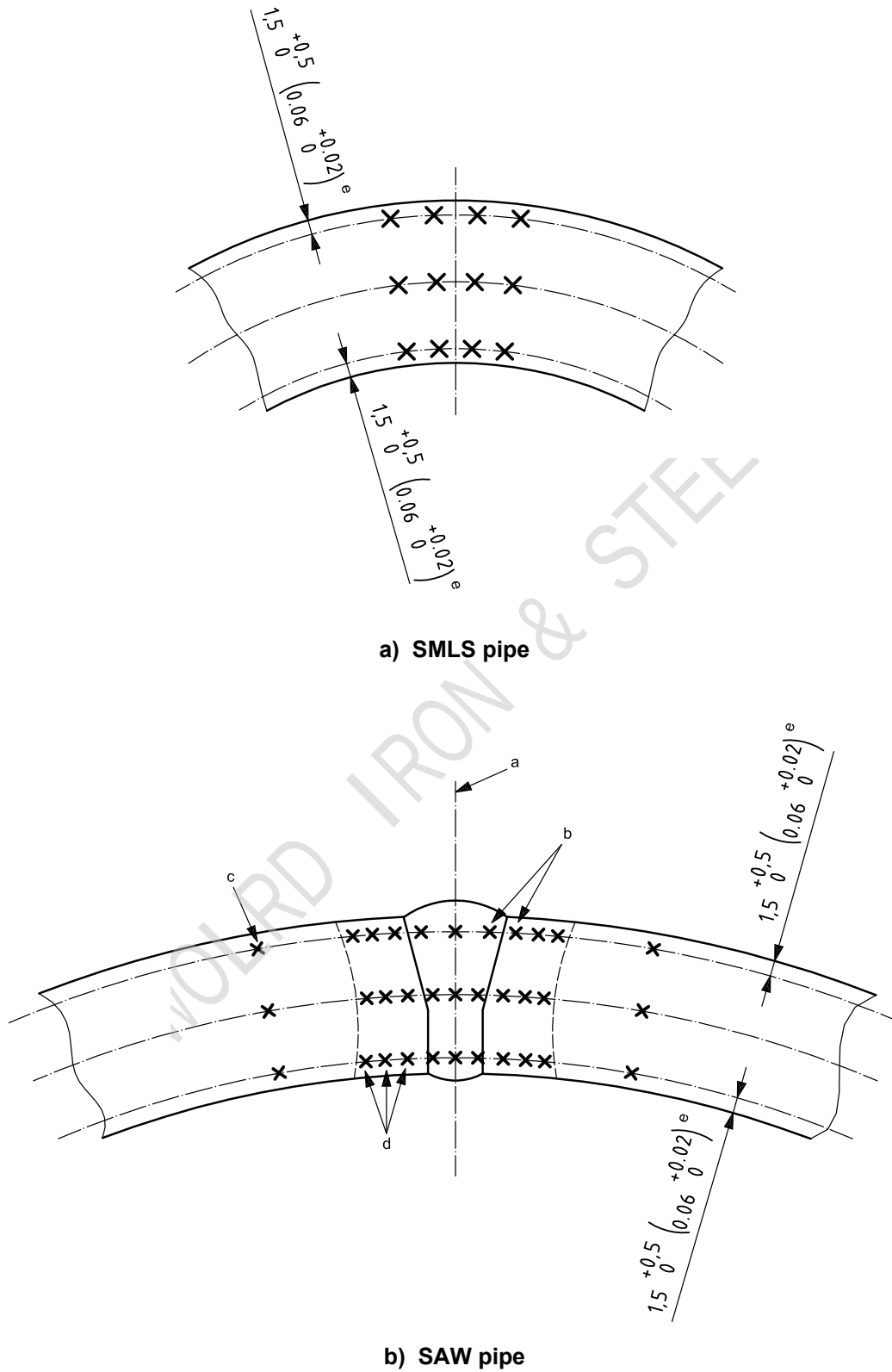
Figure H.1 — Location of hardness tests
