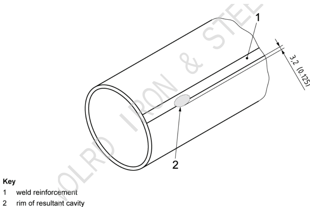
Figure C.1 — Resultant cavity of weld repair (PSL 2 only)
