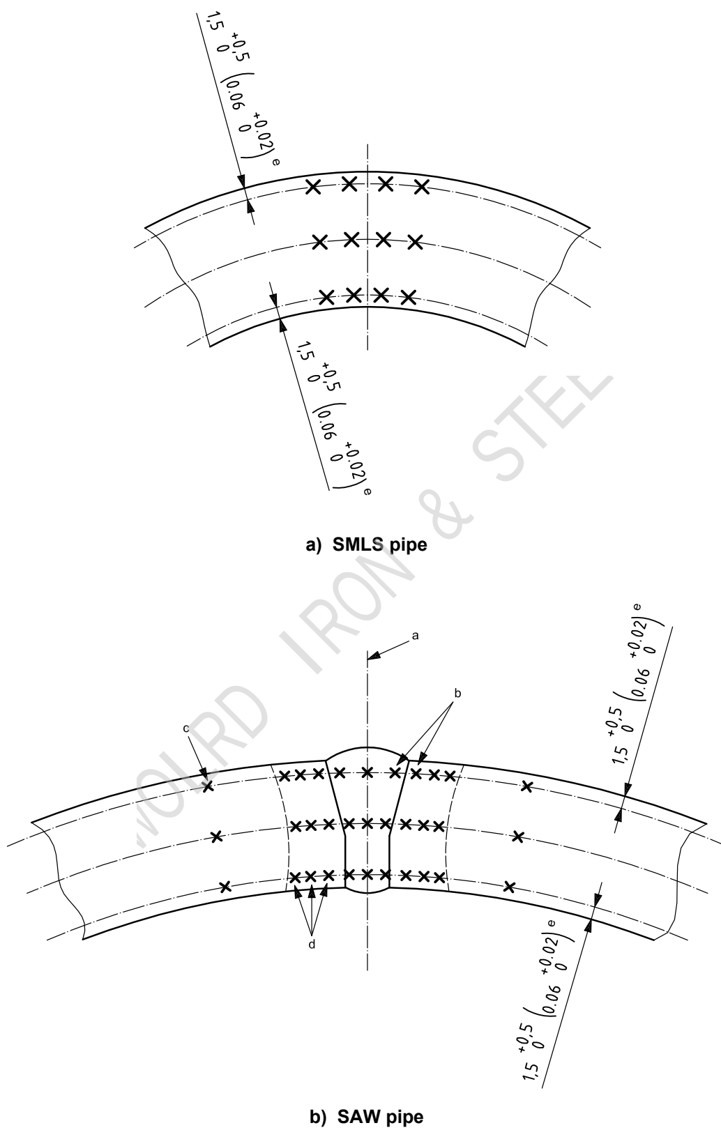
Figure J.1 — Location of hardness tests
