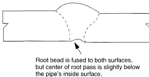
Figure 18—Internal Concavity (IC)
