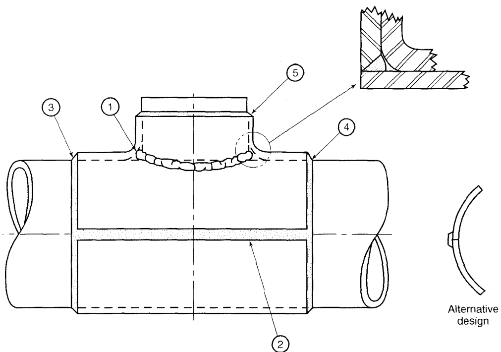
Figure B-11—Encirclement Saddle
