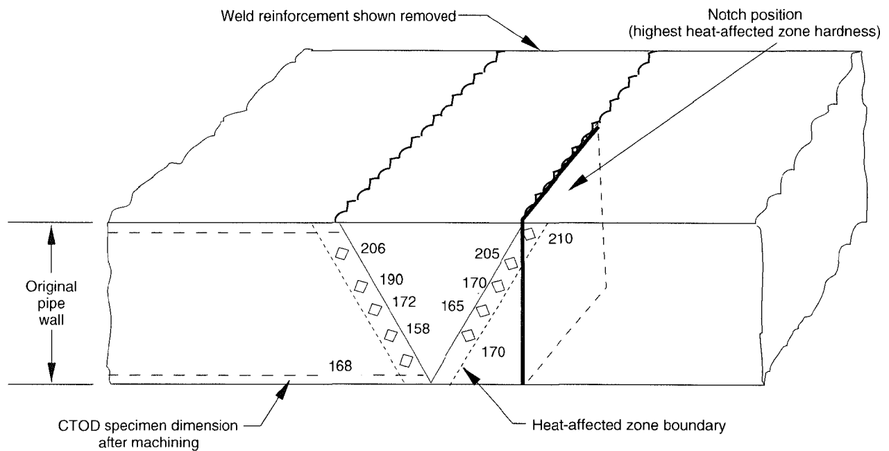
Figure A-4—Location of Notch for Heat-Affected Zone Specimen
